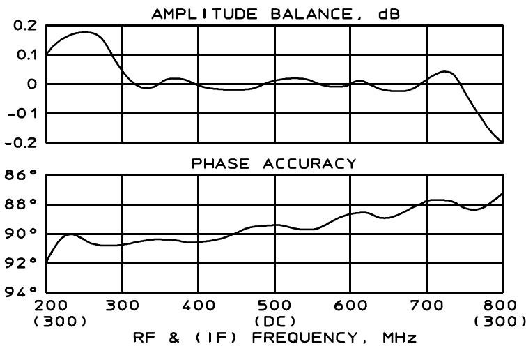
Performance over Video Bandwidth (LO at 500 MHz)
